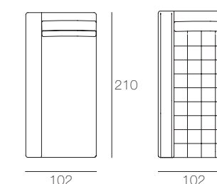
Panca sx/dx_Bench left/right
